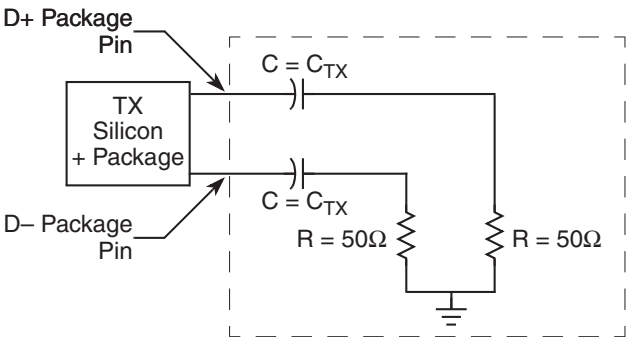
Figure 2-40. SGMII AC Test/Measurement Load
