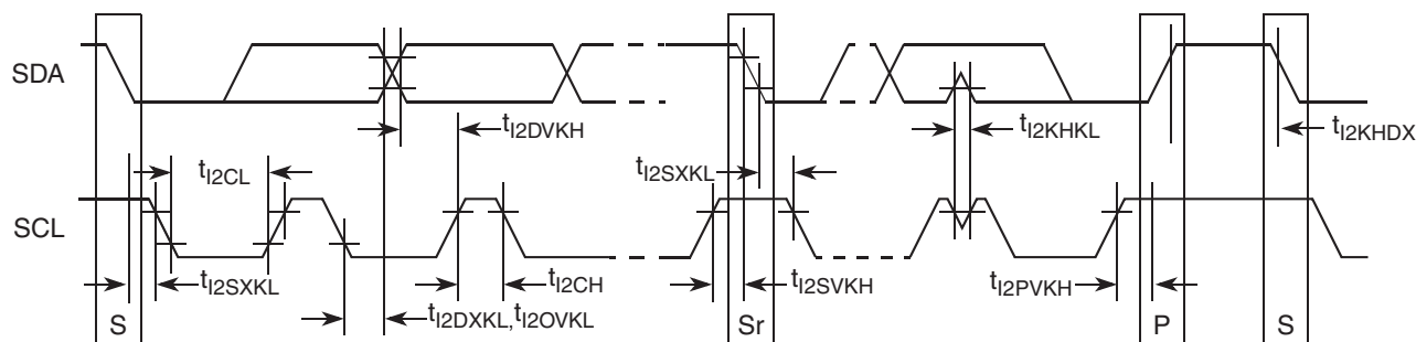
Figure 2-24. I 2 C Bus AC Timing Diagram
