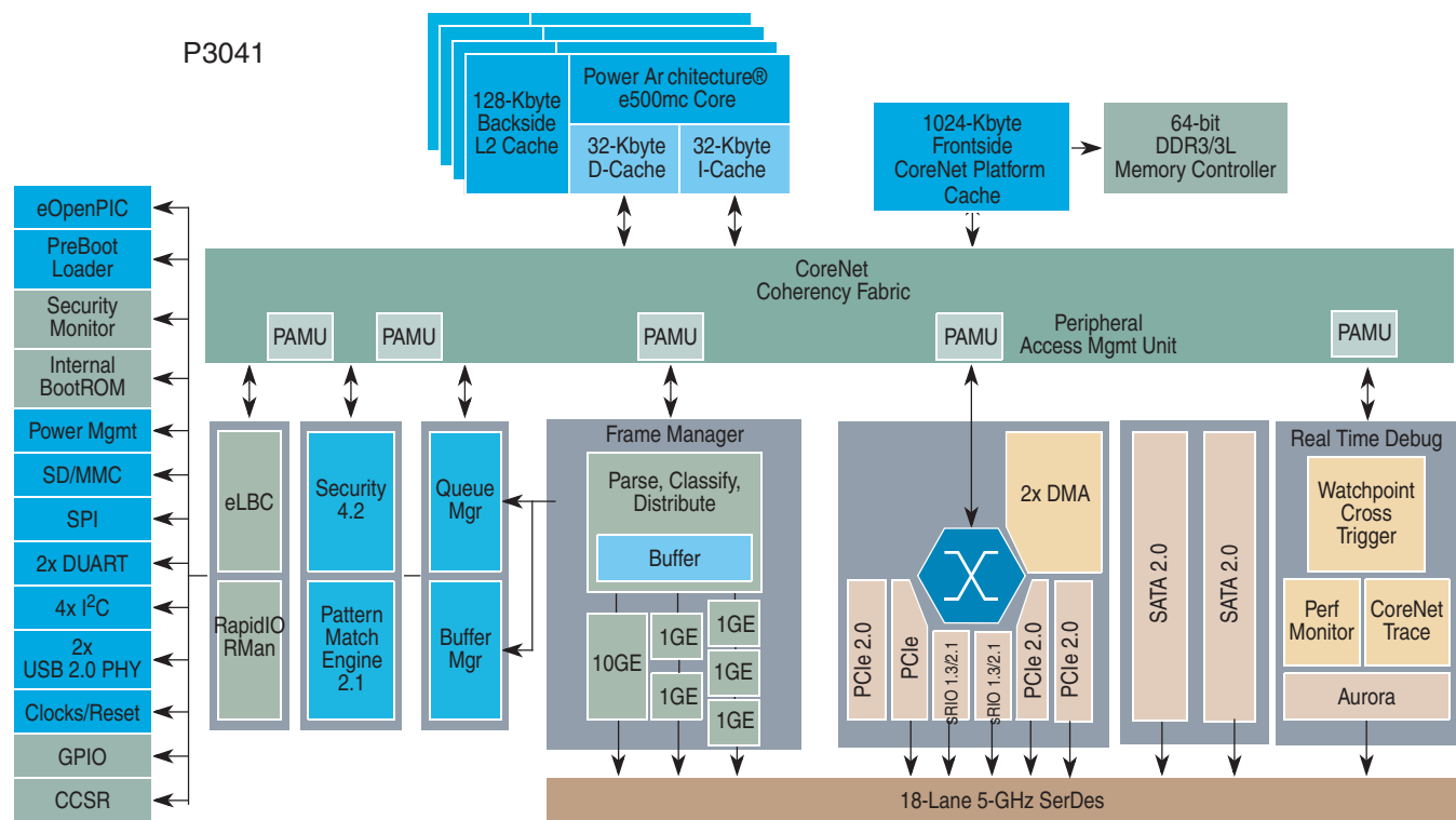
Figure 0-1. Block Diagram
