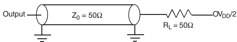
Figure 2-25. GPIO AC Test Load
