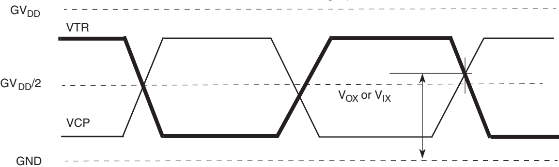
Figure 2-7. DDR3 and DDR3L SDRAM Differential Timing Specifications
