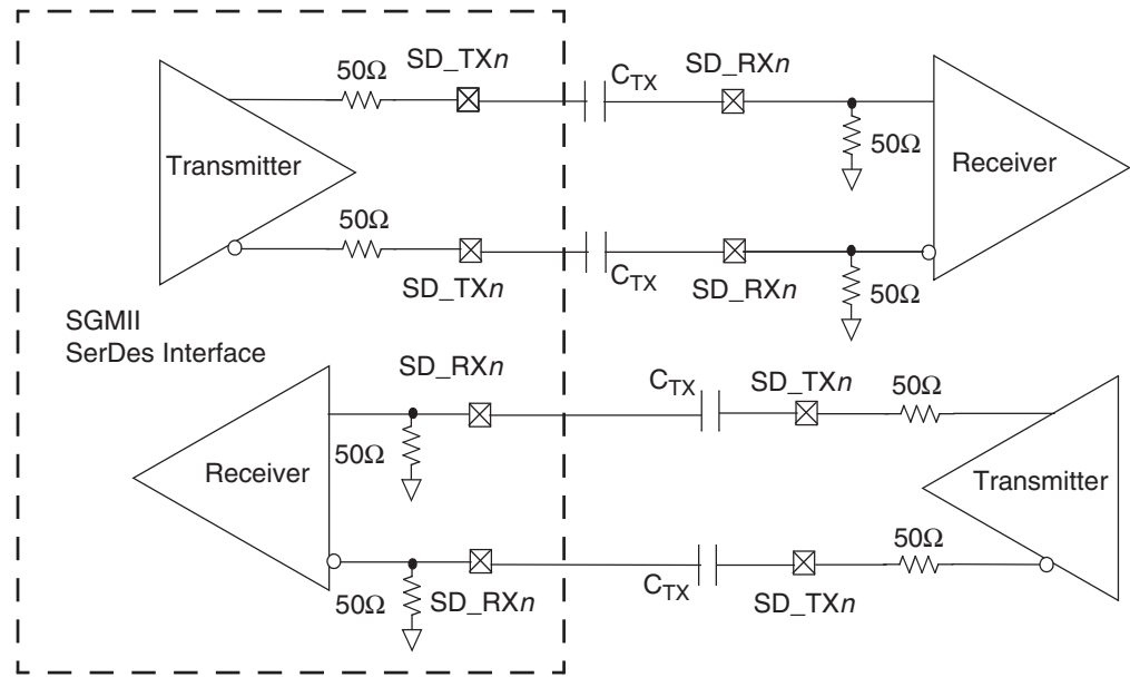
Figure 2-38. 4-Wire AC-Coupled SGMII Serial Link Connection Example
