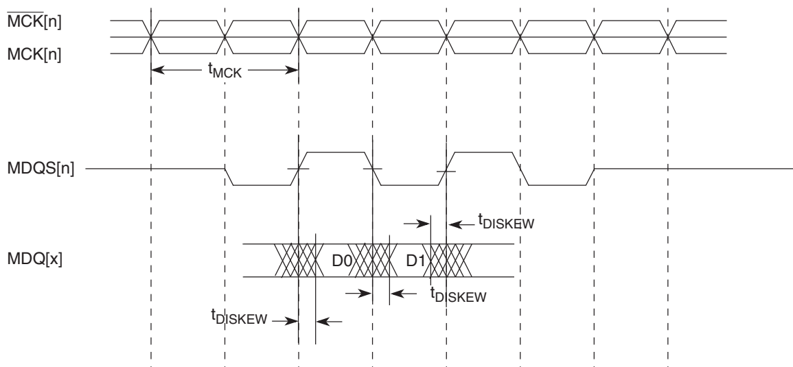
Figure 2-3. DDR3 and DDR3L SDRAM Interface Input Timing Diagram
