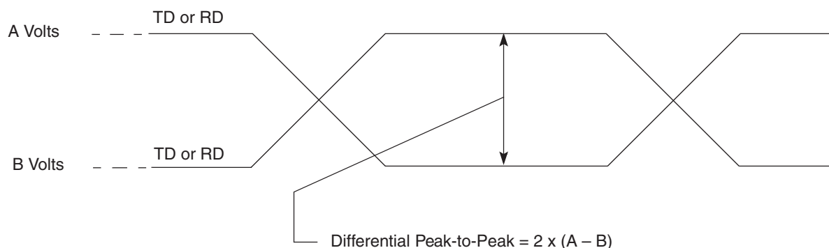
Figure 2-35. Differential Peak-to-Peak Voltage of Transmitter or Receiver
