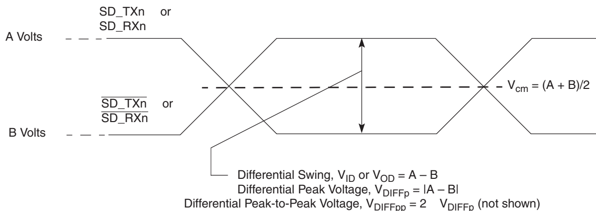
Figure 2-26. Differential Voltage Definitions for Transmitter or Receiver
