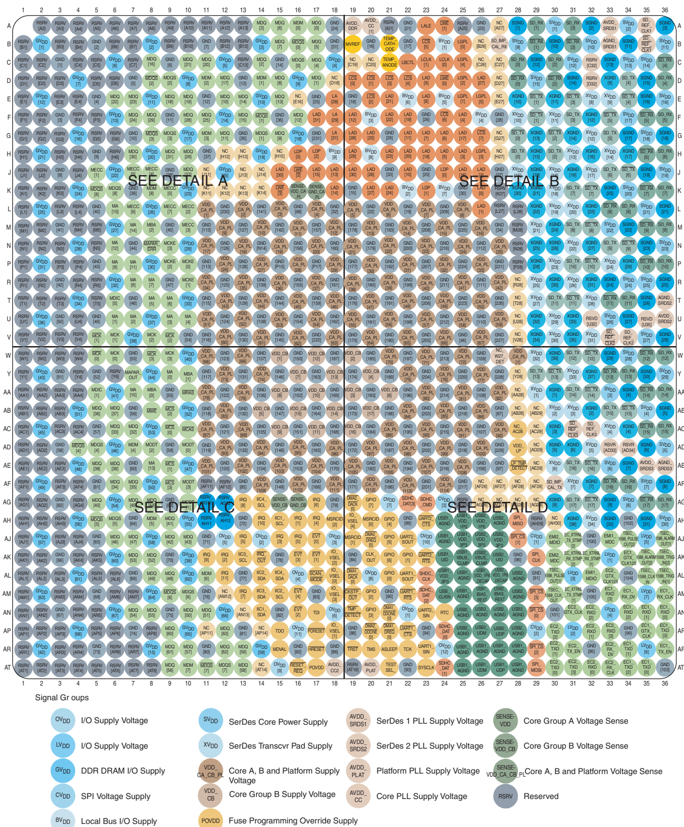
Figure 1-1. 1295 BGA Ball Map Diagram (Top View)
