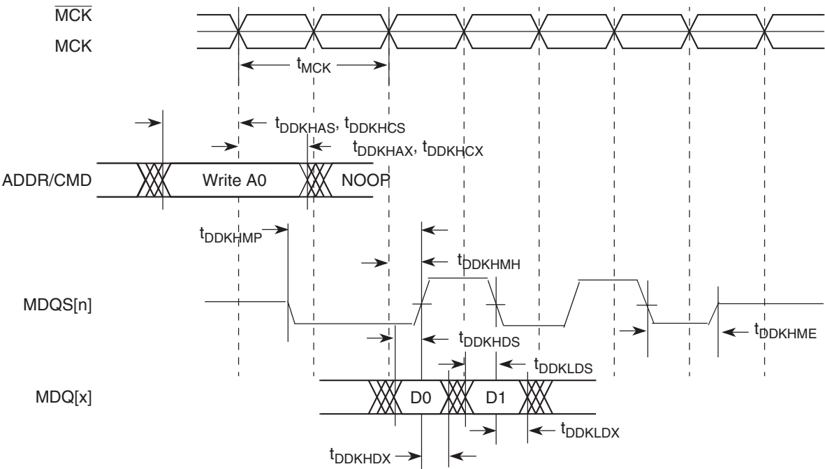
Figure 2-5. DDR3 and DDR3L Output Timing Diagram
